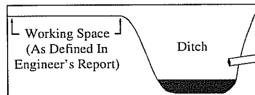
FIGURE 2. Cross-Section of an Open Ditch Municipal Drain
