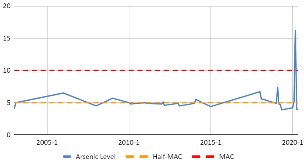
Ripley Pumphouse - Historical Arsenic (ug/L)
