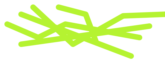
Branches
